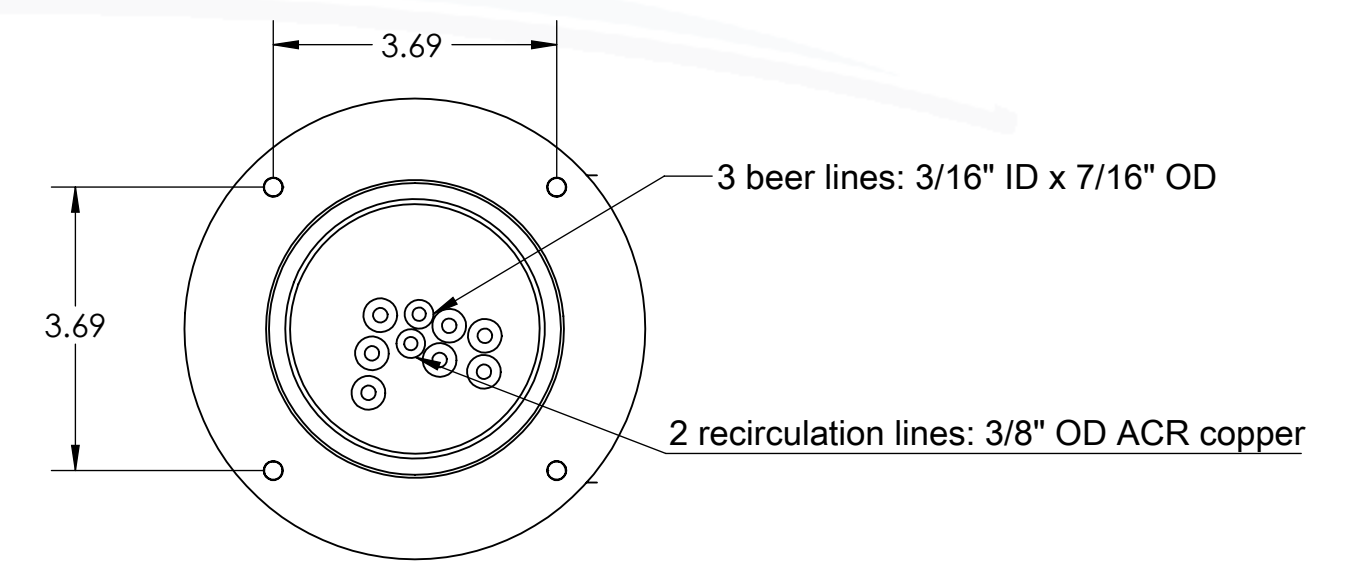
DETAIL A SCALE 2 : 5
